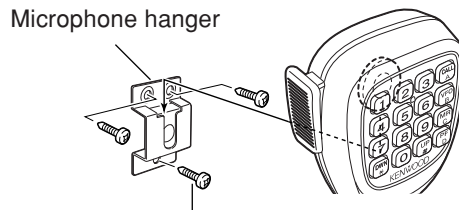
Microphone hanger screw (3 mm x 10 mm)
